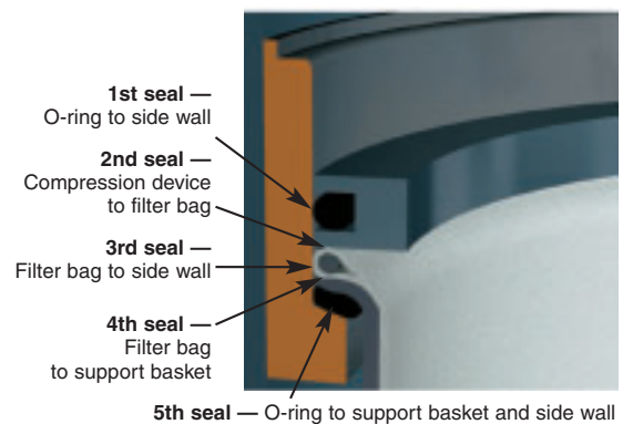
Vessel Under Compression
